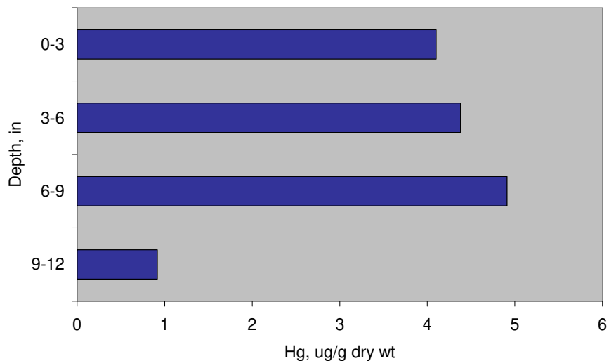
Soil Sample Location 015
