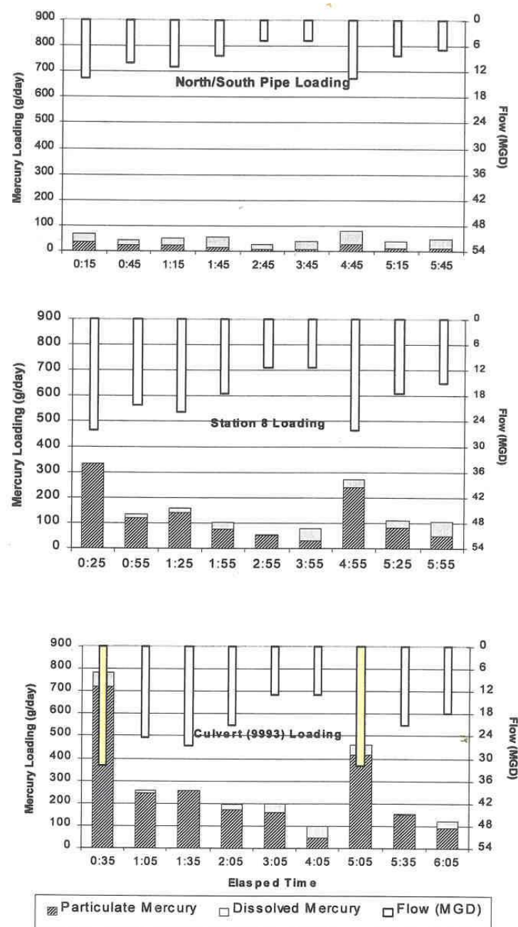
Fig. 3.15. Dissolved and particulate mercury loading in UEFPC during a storm on January 7, 1998.
